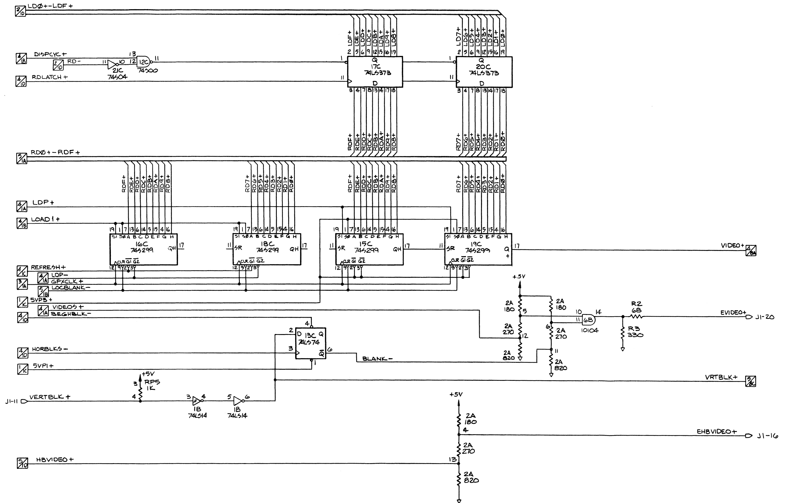
Figure 3-2. IWS Graphics Control Board Schematic. (Page 7 of 7)
