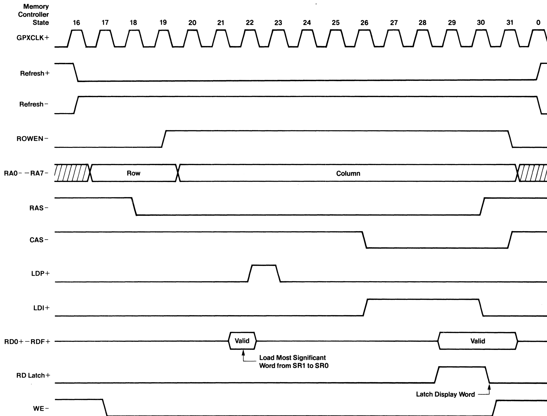
Figure 3-5. Display Memory Access Timing Diagram.
